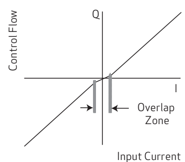
Overlap Spool
